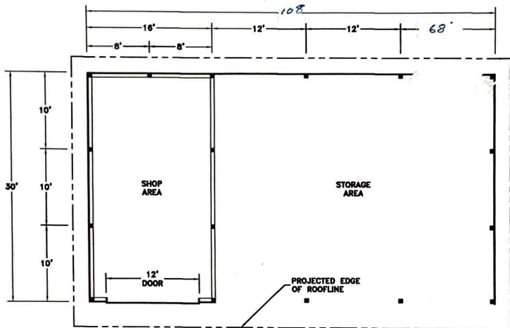
PLAN SCALE: 3/32" = 1'-0"
