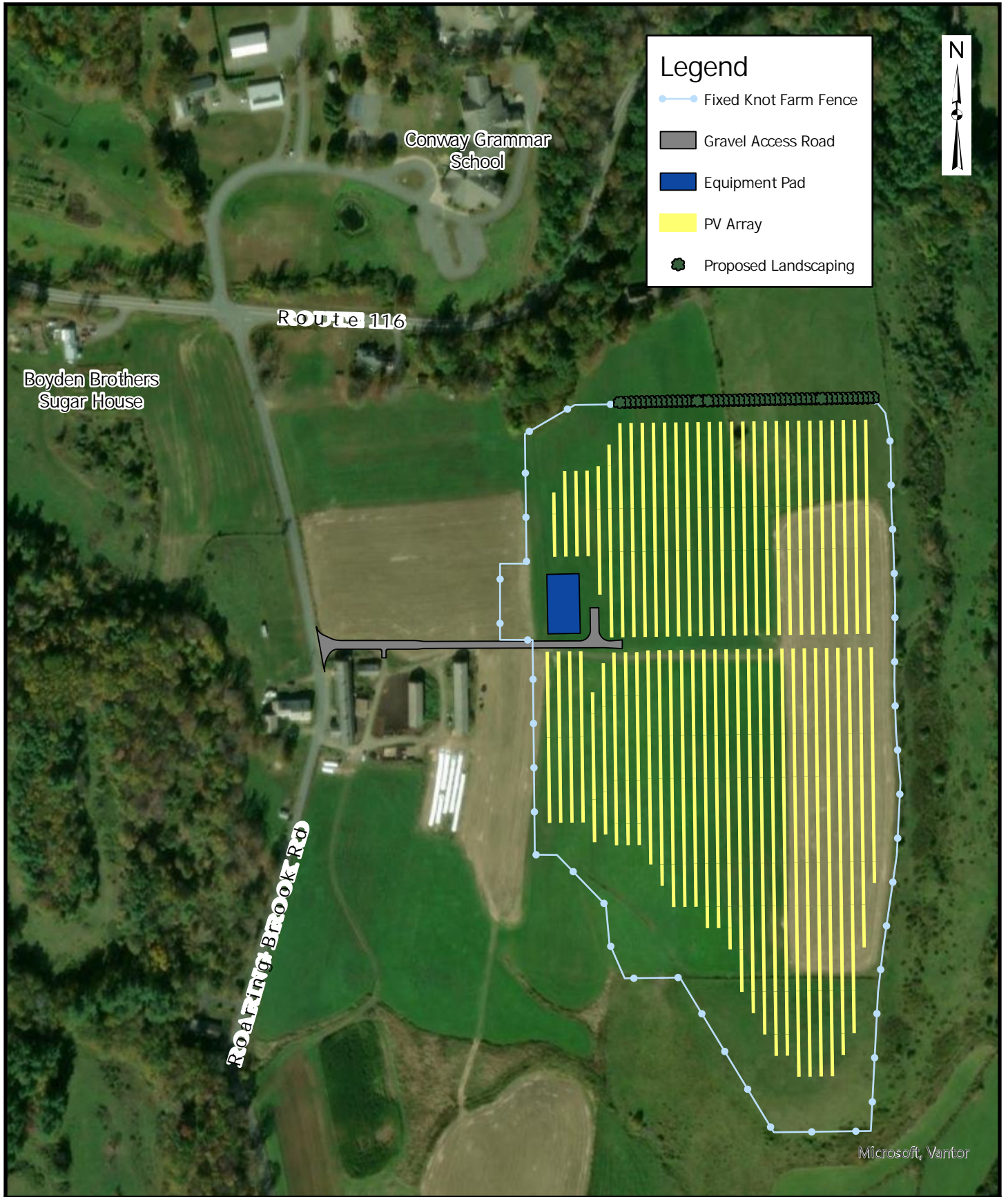
FIGURE 1 CONWAY SOLAR PV DEVELOPMENT MAP 412 LOT 8, ROARING BROOK ROAD CONWAY MA
